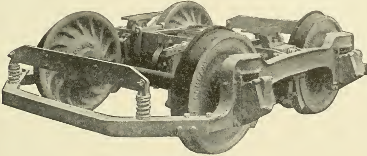
Fig. 14. Short Wheel-Base Truck
